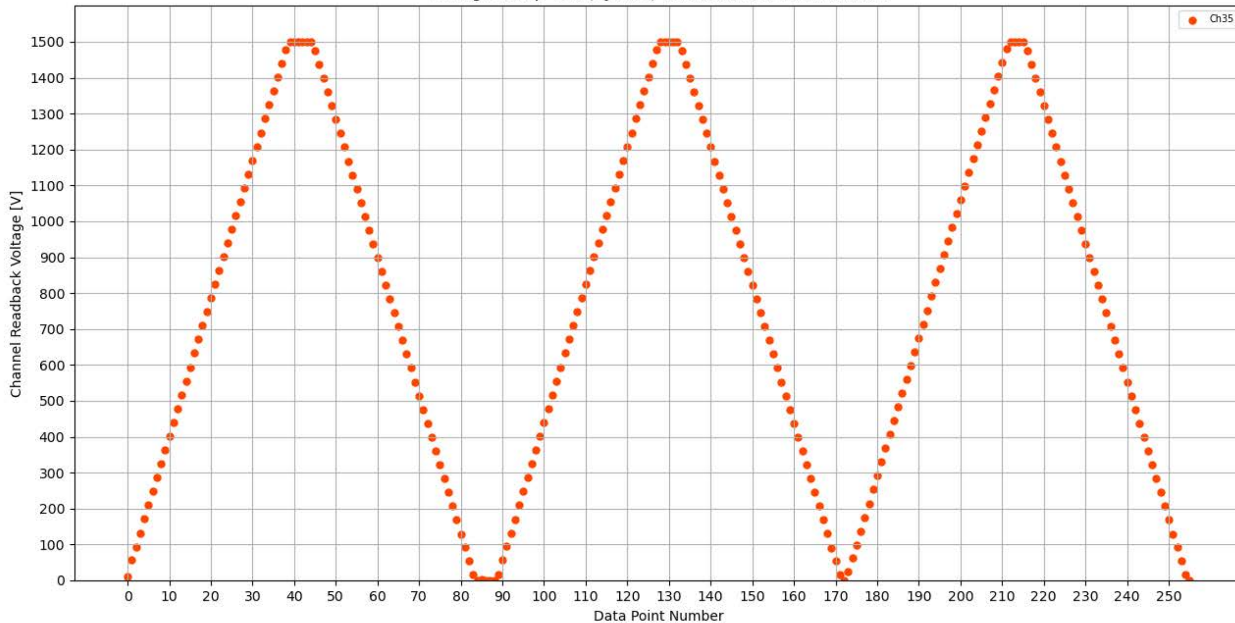
Voltage Ramp Test (Python) Bd #262, Slot #11, Ch #35
