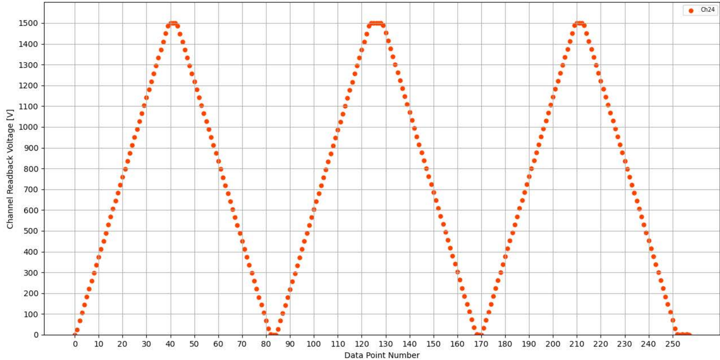
Voltage Ramp Test (Python) Bd #262, Slot #11, Ch #24
