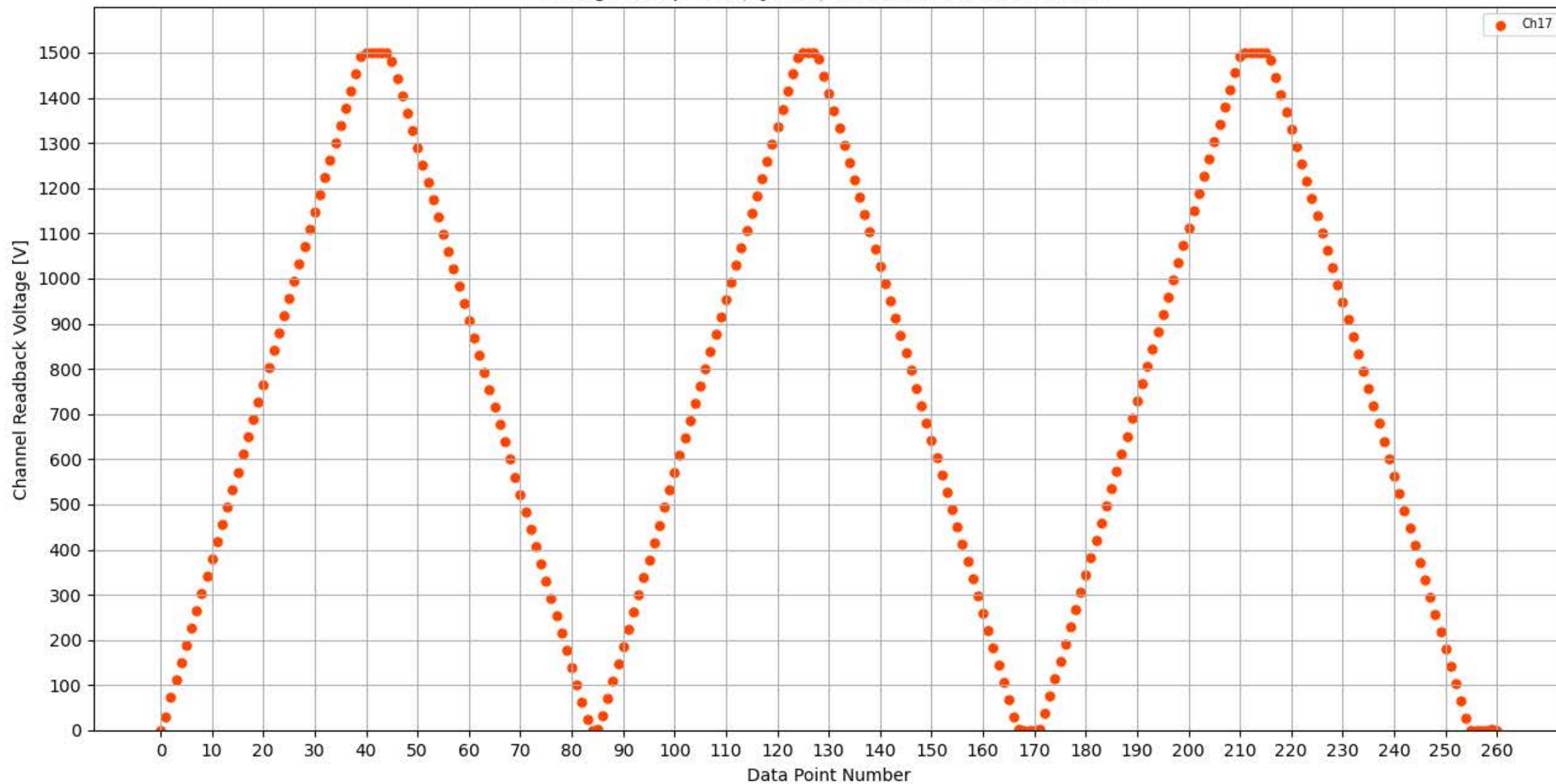
Voltage Ramp Test (Python) Bd #262, Slot #11, Ch #17
