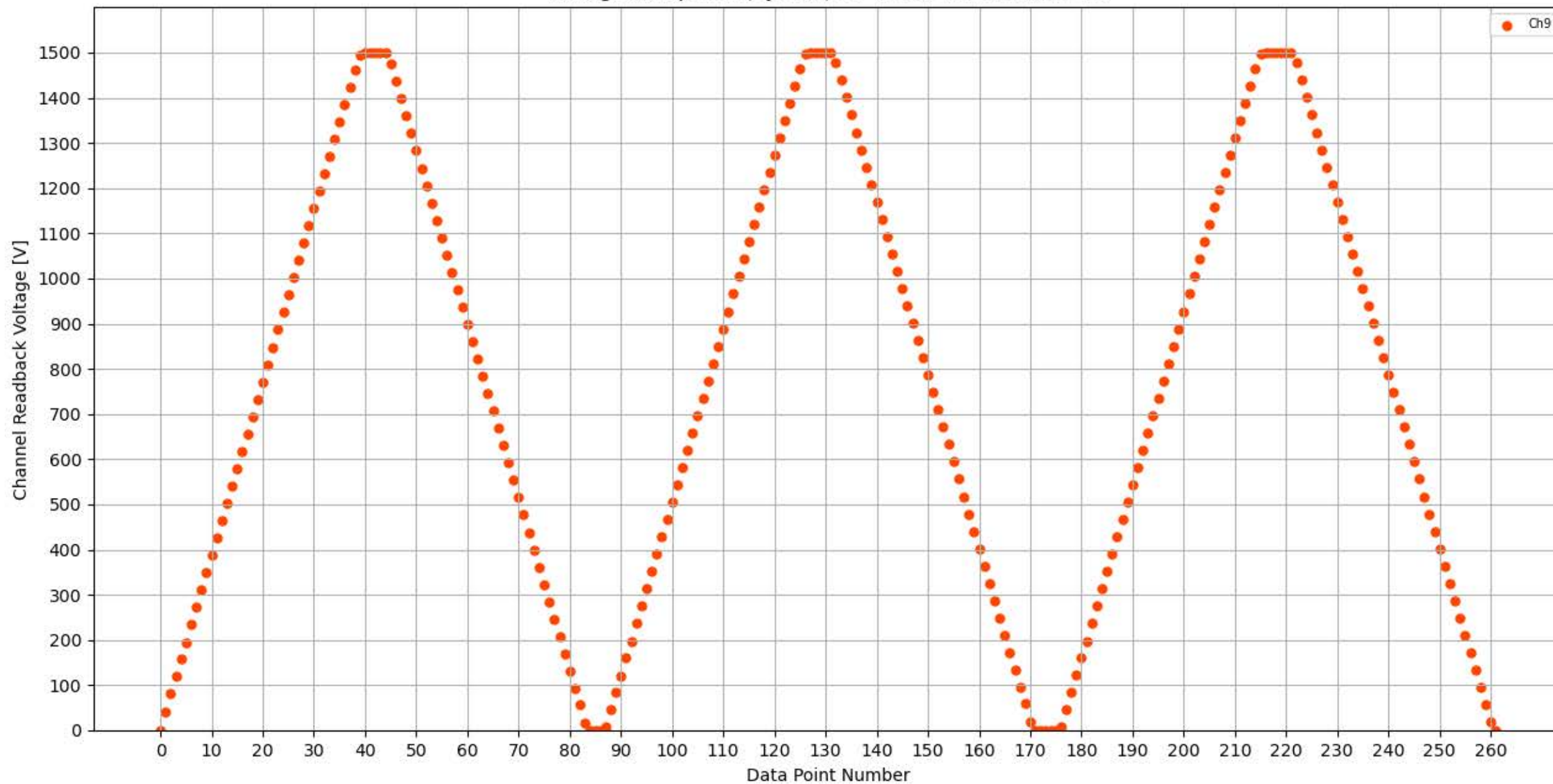
Voltage Ramp Test (Python) Bd #262, Slot #11, Ch #9
