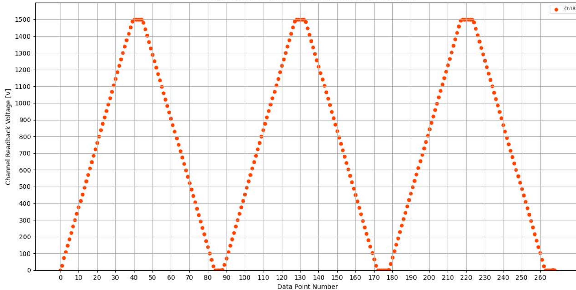
Voltage Ramp Test (Python) Bd #262, Slot #11, Ch #18
