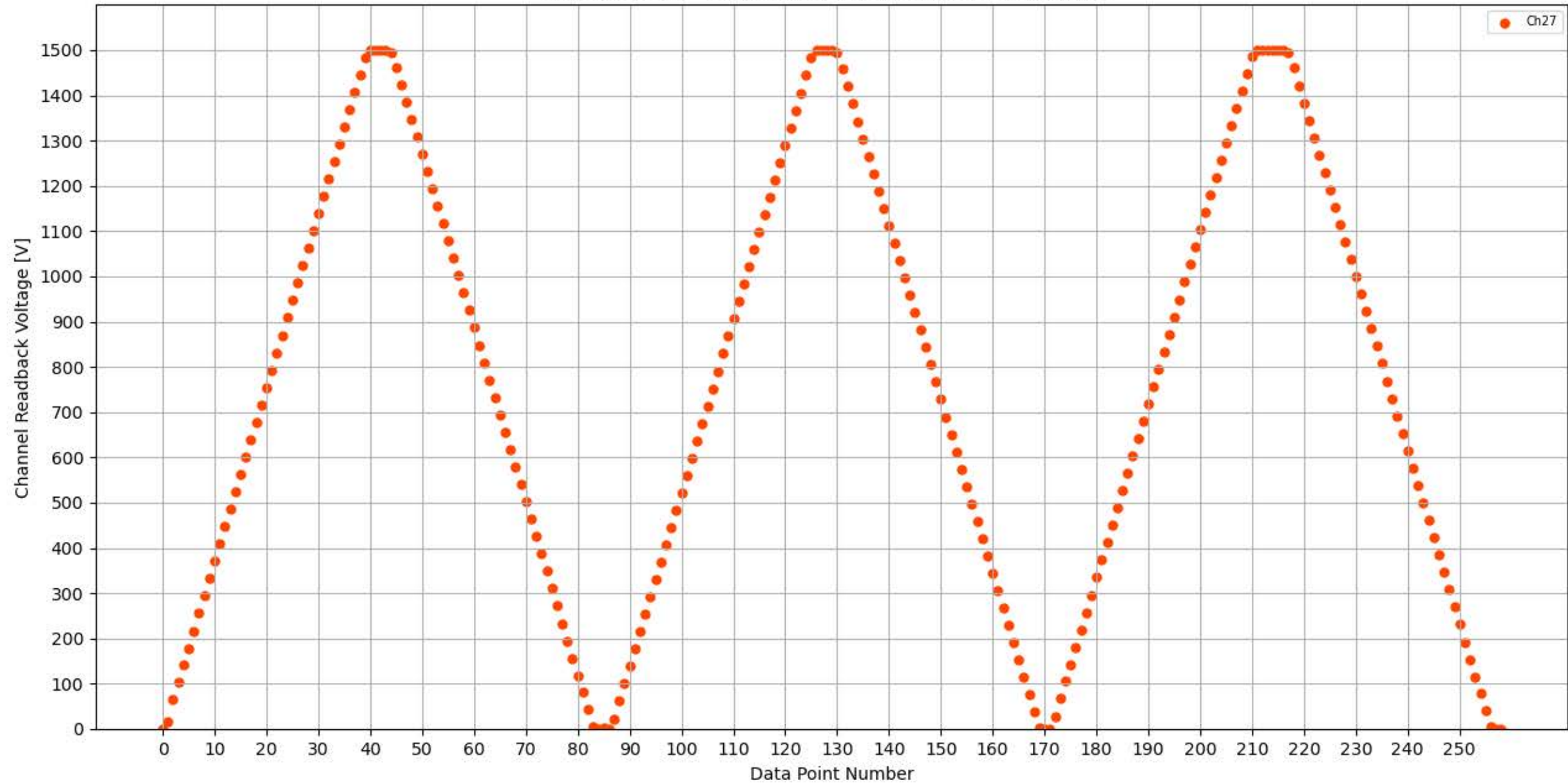
Voltage Ramp Test (Python) Bd #262, Slot #11, Ch #27
