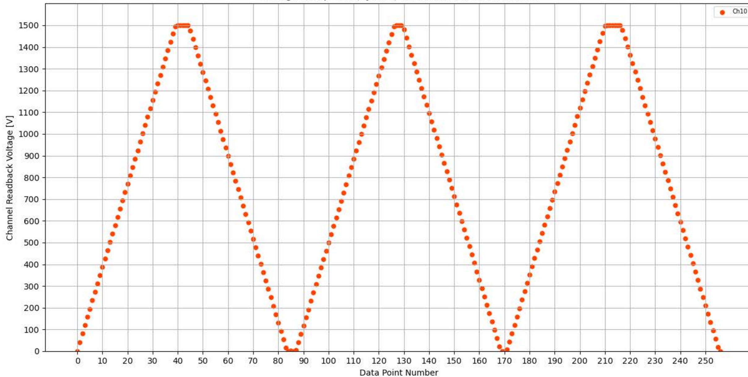
Voltage Ramp Test (Python) Bd #262, Slot #11, Ch #10
