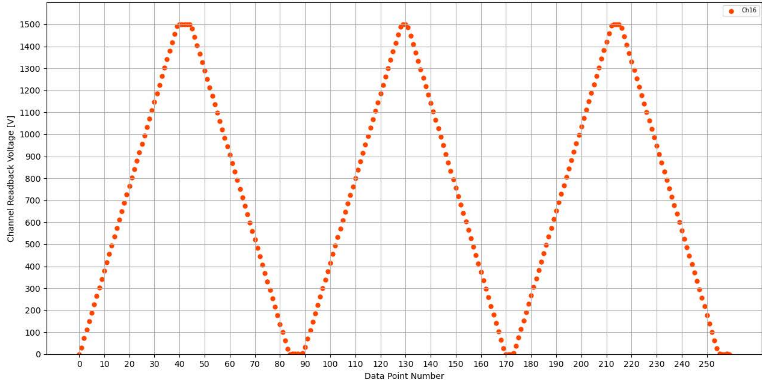
Voltage Ramp Test (Python) Bd #262, Slot #11, Ch #16
