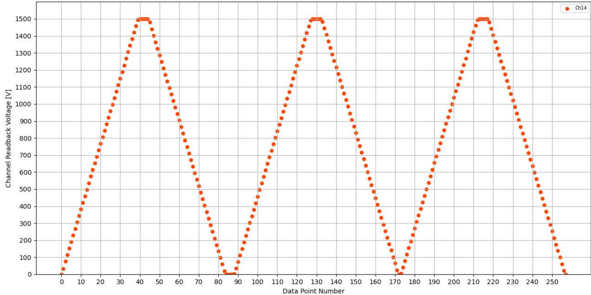
Voltage Ramp Test (Python) Bd #262, Slot #11, Ch #14
