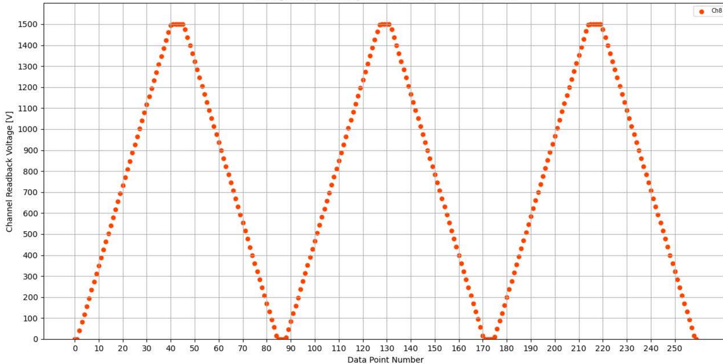
Voltage Ramp Test (Python) Bd #262, Slot #11, Ch #8
