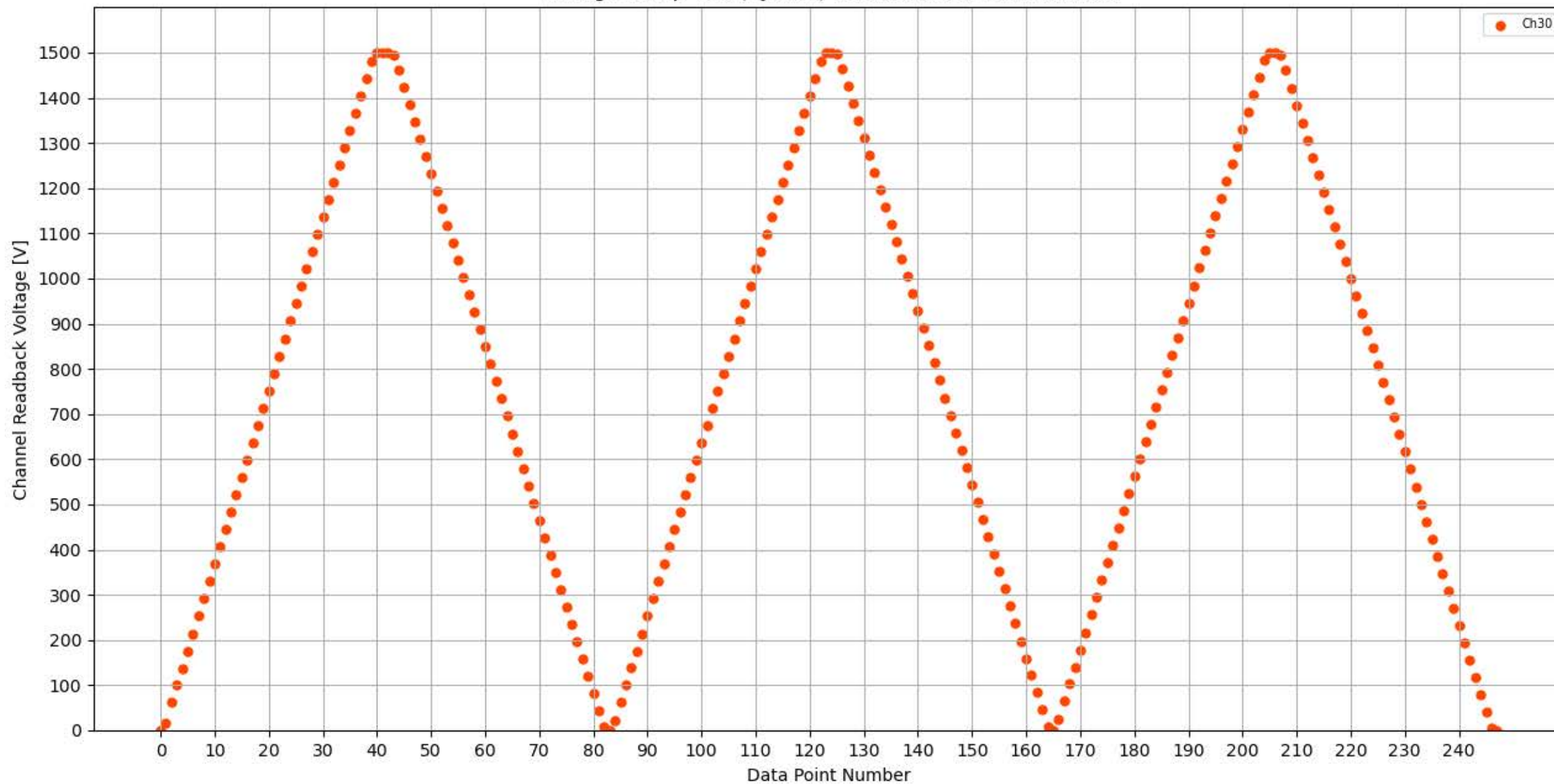
Voltage Ramp Test (Python) Bd #262, Slot #11, Ch #30
