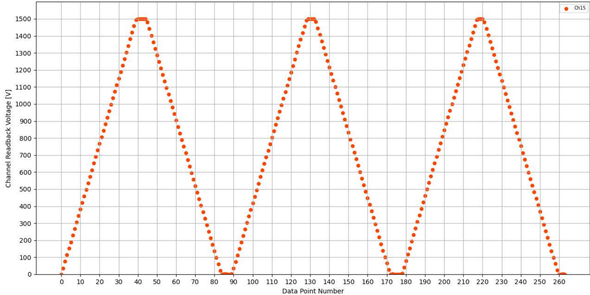
Voltage Ramp Test (Python) Bd #262, Slot #11, Ch #15
